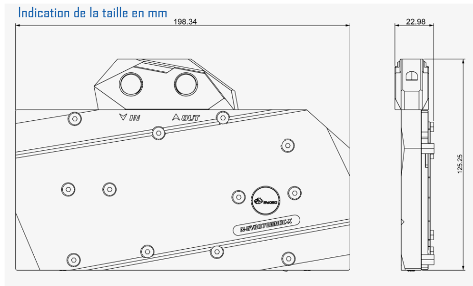
N-GV3070GMOC-X (1 pc)
