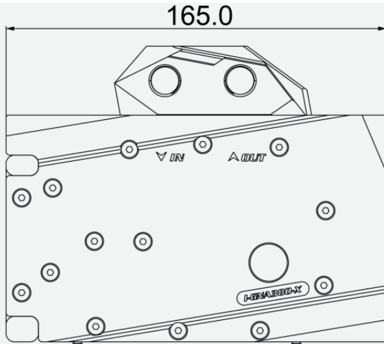
Waterblock (1 pc)
