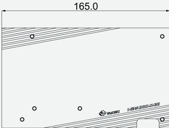
Backplate (1 pc)
